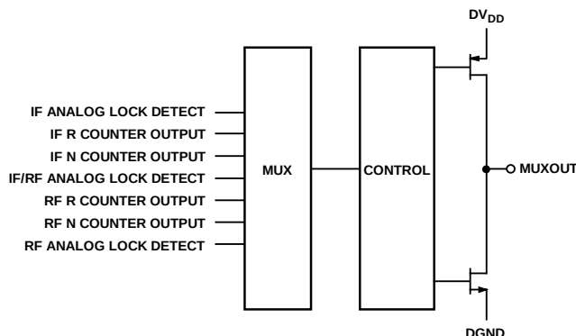
Figure 30. MUXOUT Schematic
