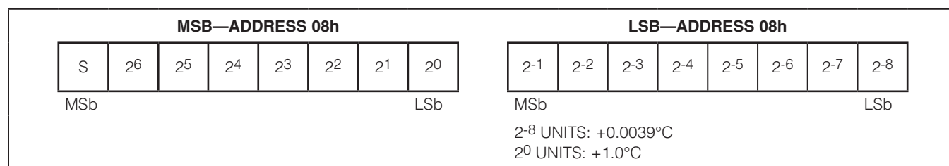
Figure 58. Temperature Register Format (Input/Output)
