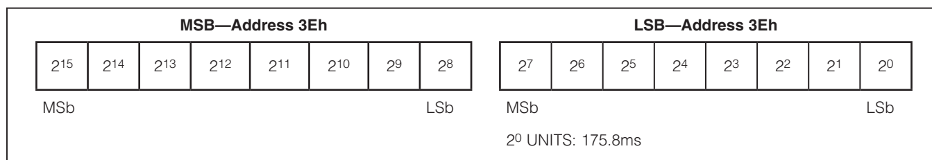
Figure 45. Timer Register Format (Output)
