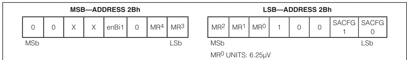
Figure 34. MiscCFG Register Format (Input)
