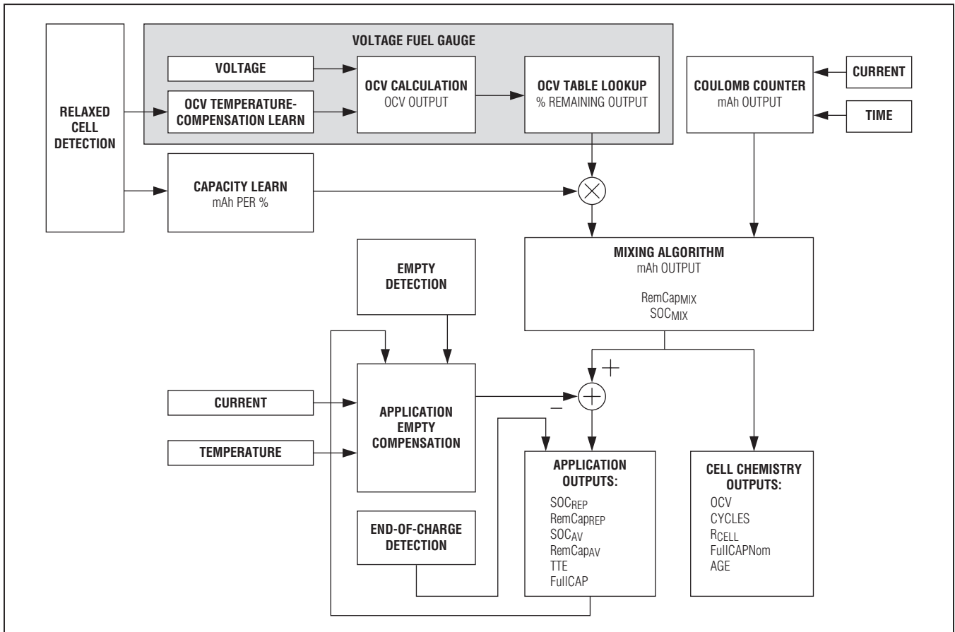
Figure 2. ModelGauge m3 Overview
