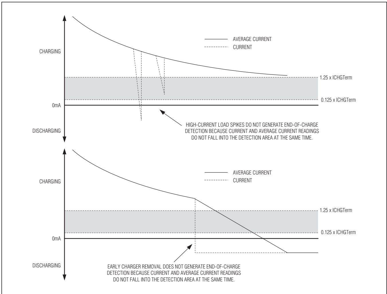
Figure 26. False End-of-Charge Events
