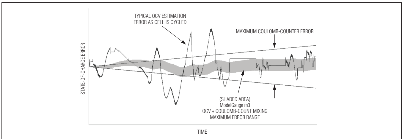
Figure 4. ModelGauge m3 Algorithm Mixing Conceptual Illustration
