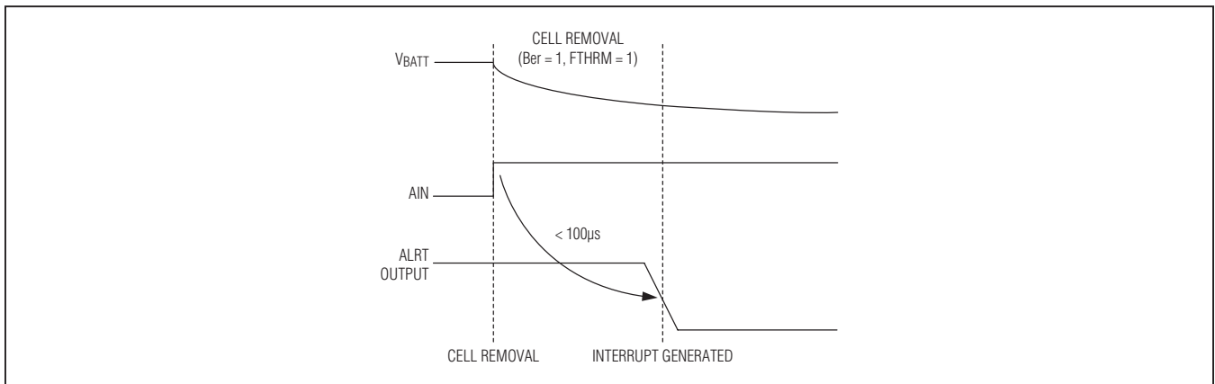
Figure 39. Fast Detection of Cell Removal
