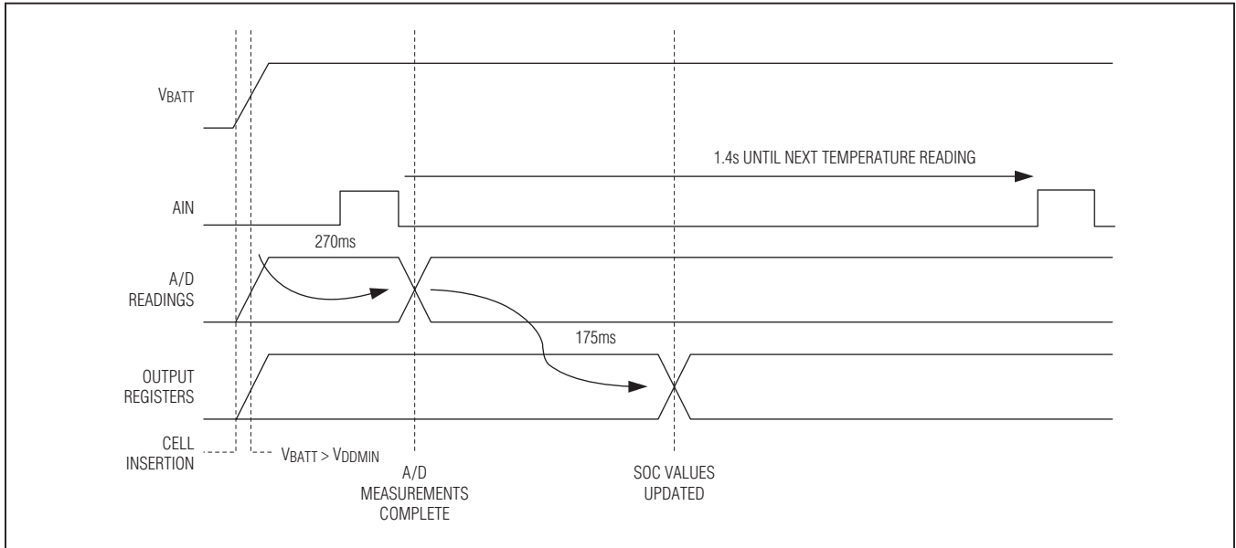
Figure 37. Power-Up Operation
