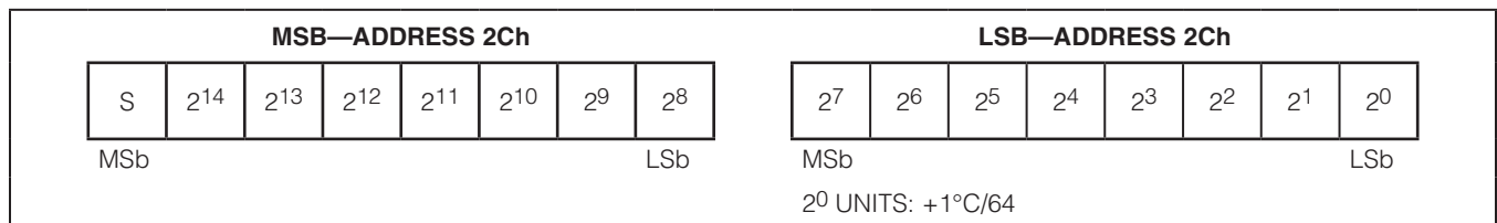
Figure 61. TGAIN Register Format (Input)
