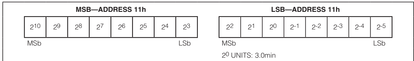
Figure 17. TTE Register Format (Output)
