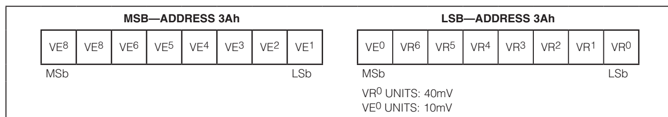
Figure 29. V_empty Register Format (Input)
