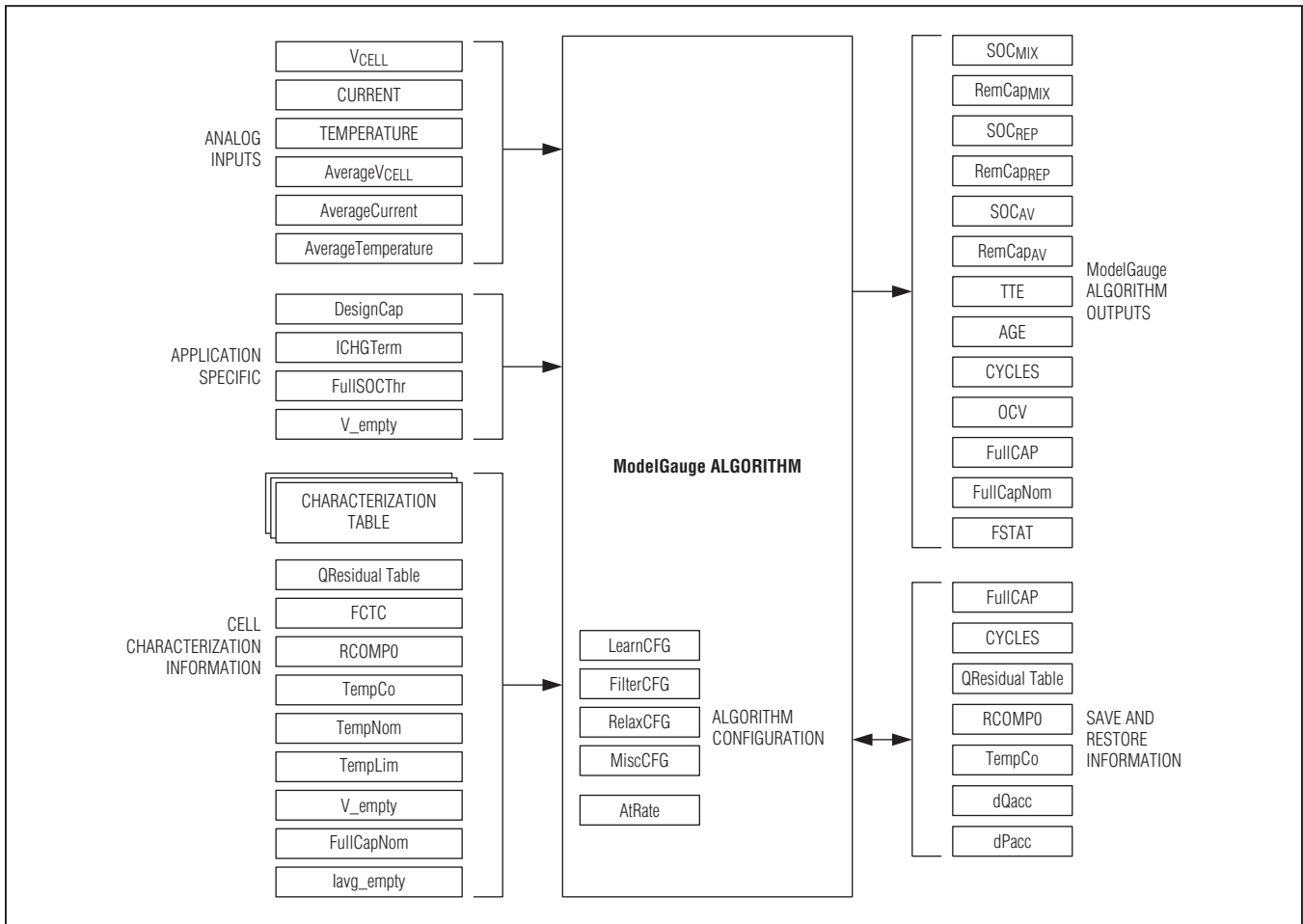
Figure 9. ModelGauge m3 Register Map
