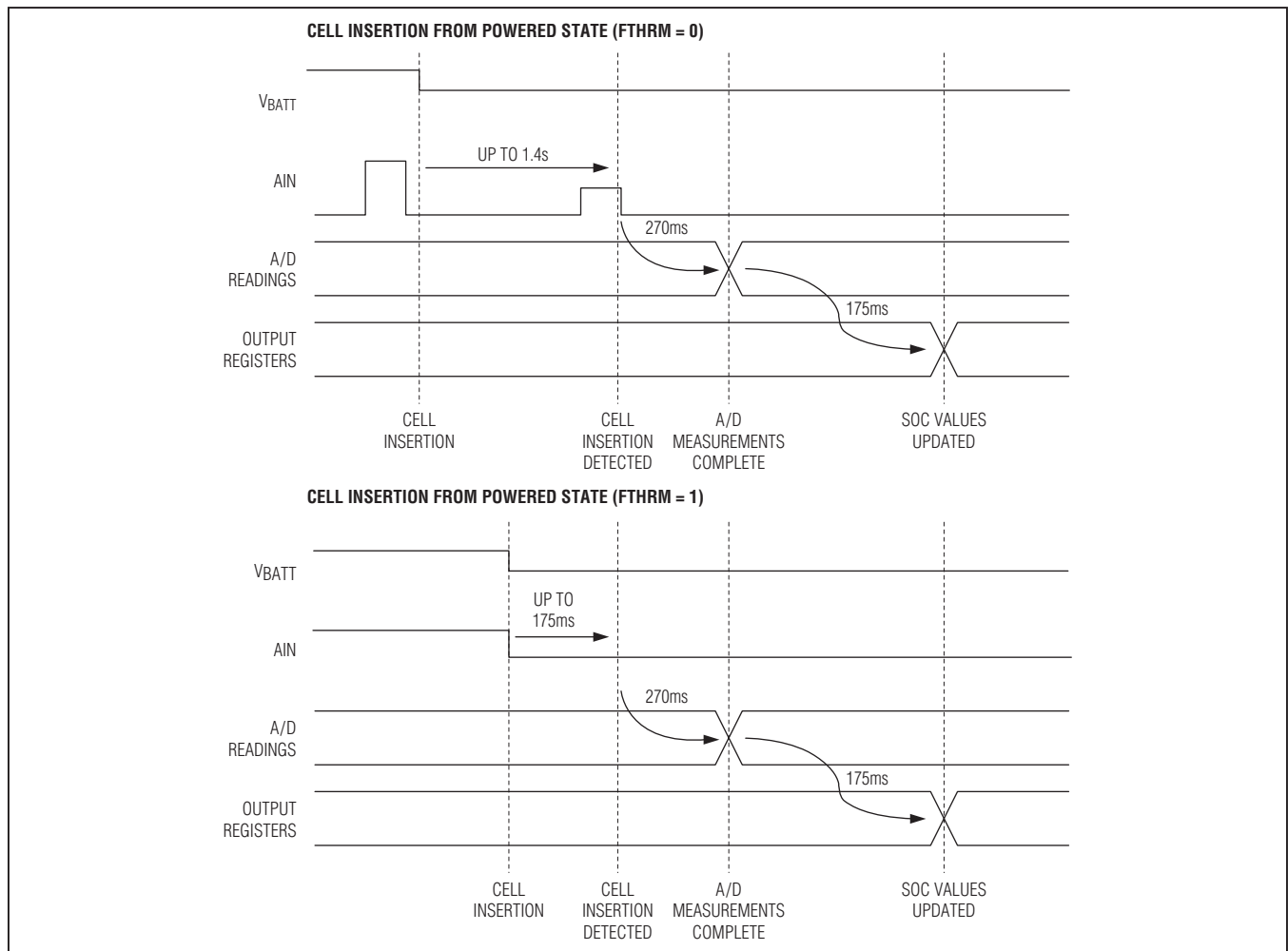
Figure 38. Operation After Cell Insertion
