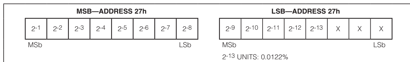
Figure 57. AIN Register Format (Output)
