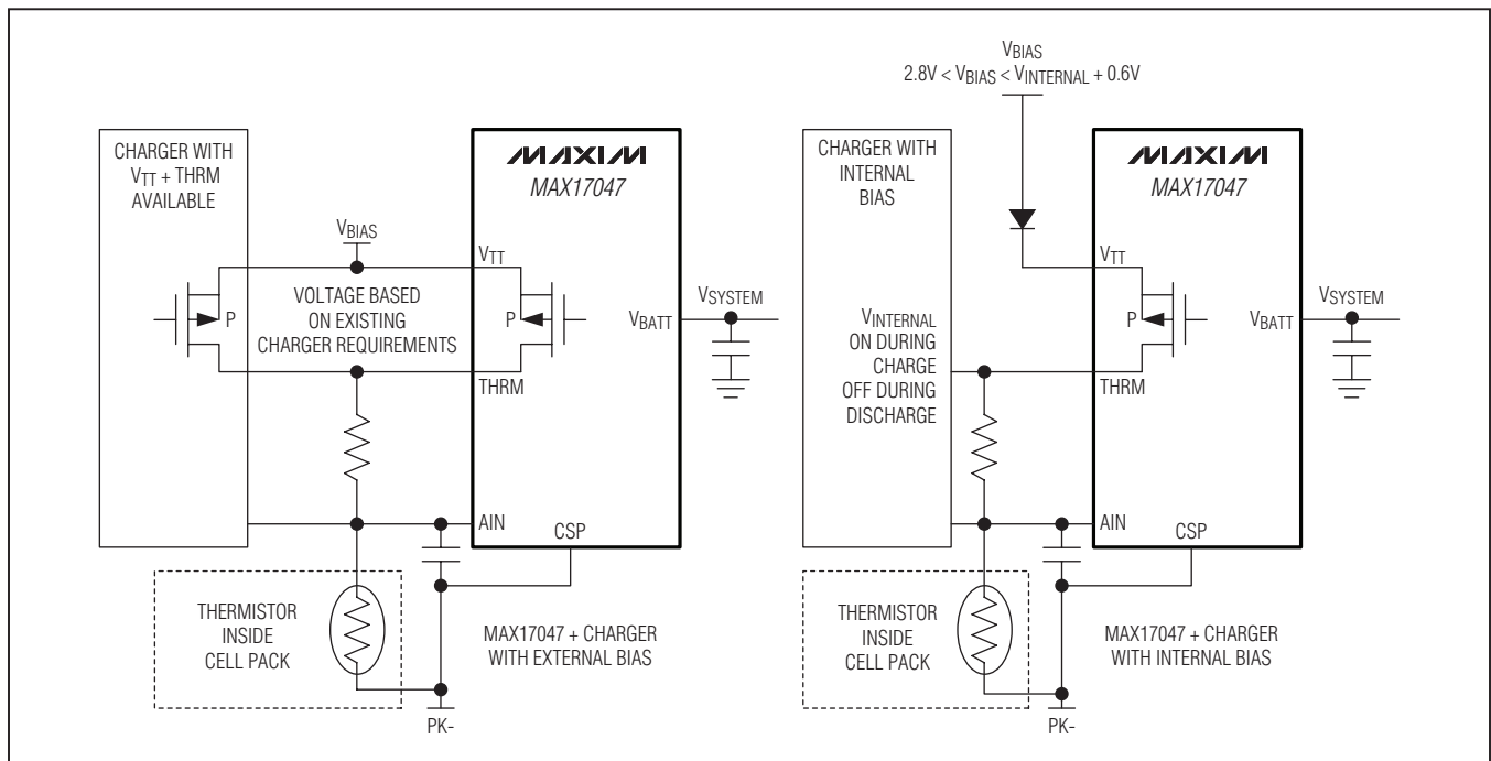
Figure 7. Operating Circuits that Share Pack Thermistor with System Charger
