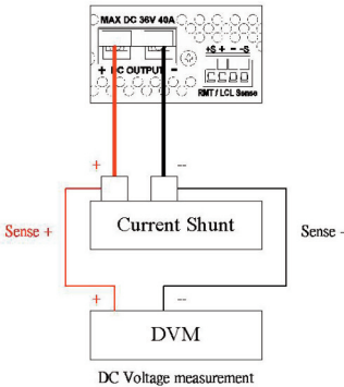
DC Voltage measurement
