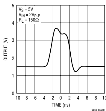
Fast Large-Signal Transient Response
