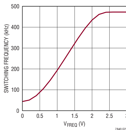
Switching Frequency vs FREQ Pin Voltage
