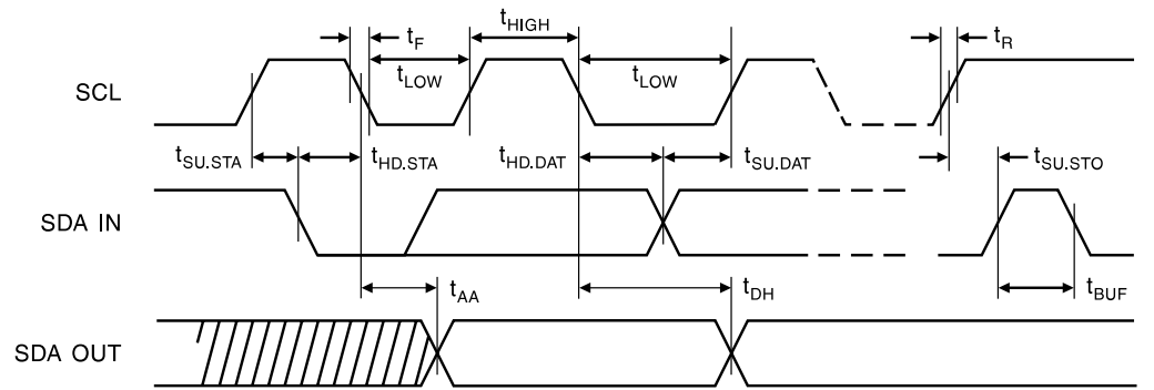
Figure 3. Bus Timing (1)
