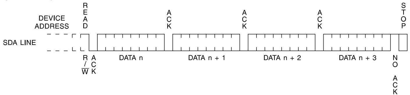
Figure 13. Sequential Read.
