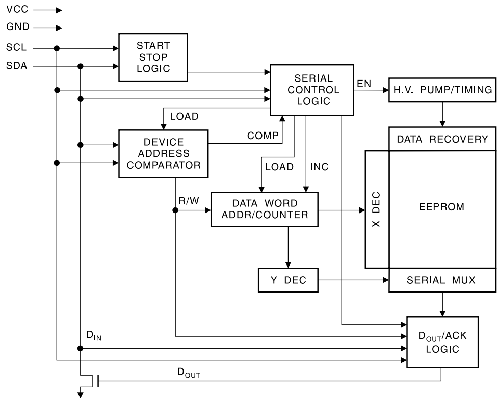
Figure 2. Block Diagram
