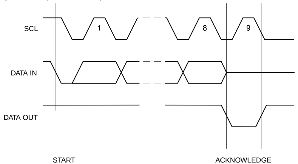
Figure 7. Output Acknowledge
