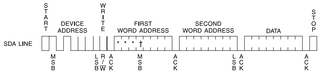
Figure 9. Byte Write
