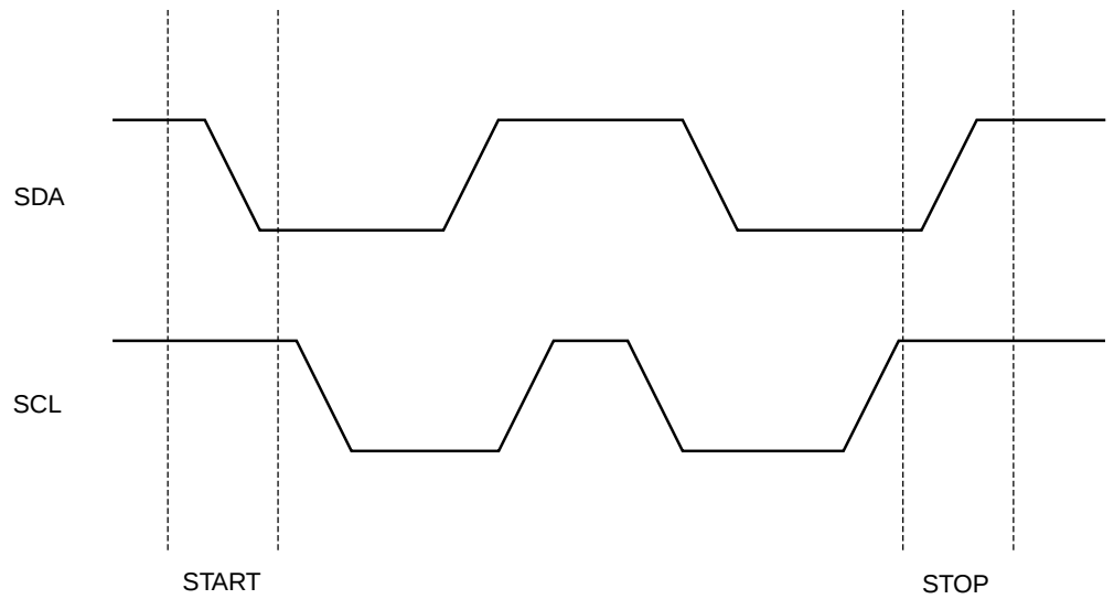
Figure 6. Start and Stop Definition
