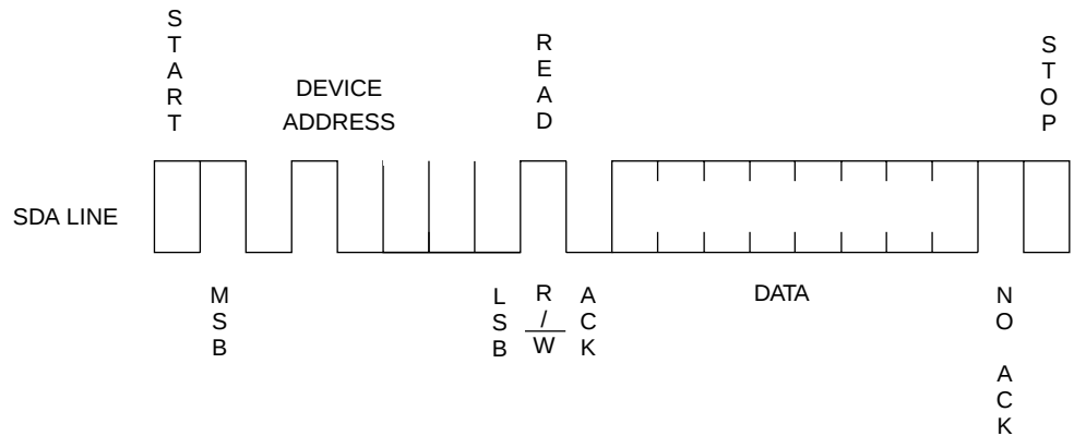
Figure 11. Current Address Read
