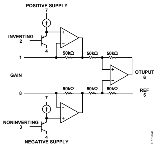
Figure 41. Simplified Schematic
