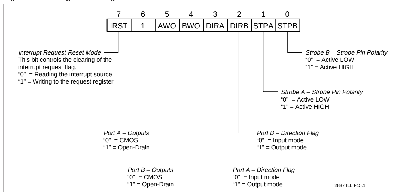
Figure 11. Configuration Register
