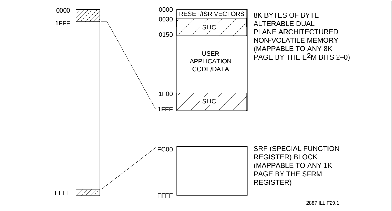
Figure 6. Microcontroller Map
