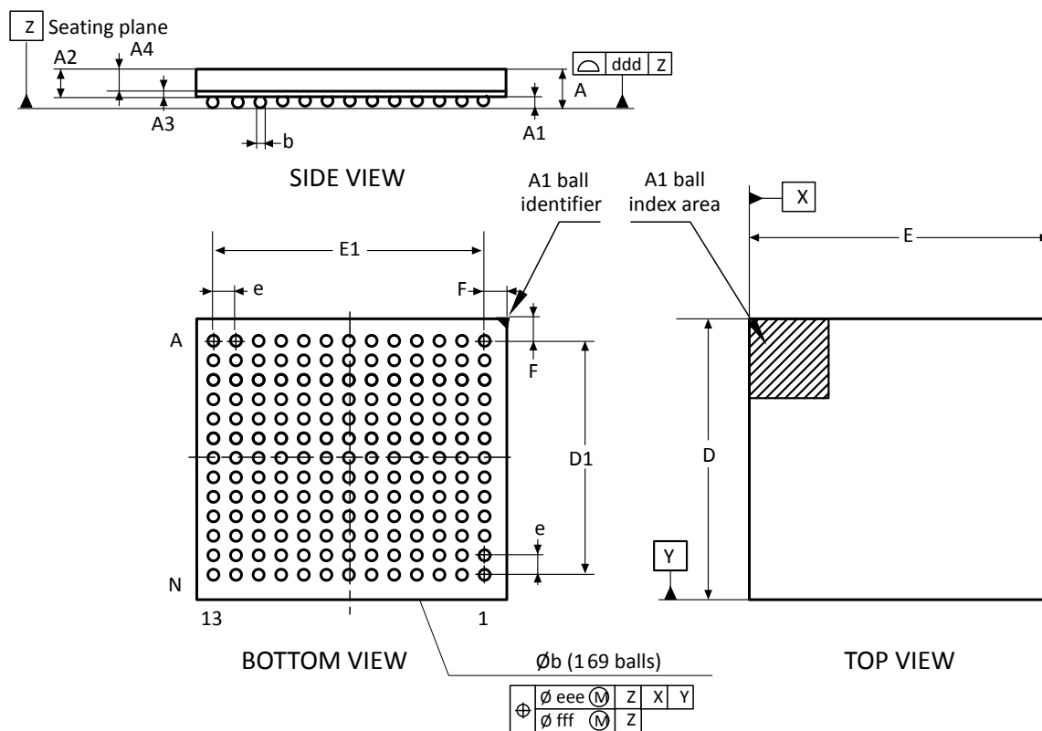
Figure 85. UFBGA169 - Outline
