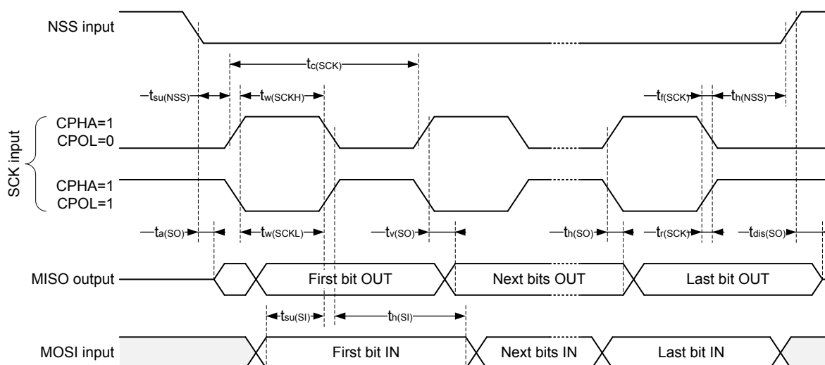
Figure 60. SPI timing diagram - slave mode and CPHA = 1 (1)
