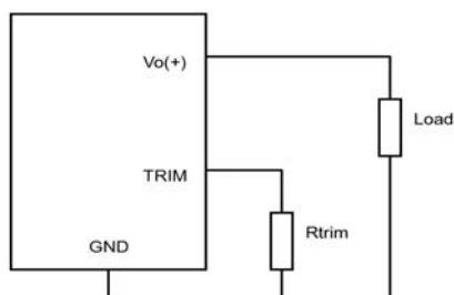
Figure 29: Trim up Circuit configuration for programming output voltage using an external resistor
