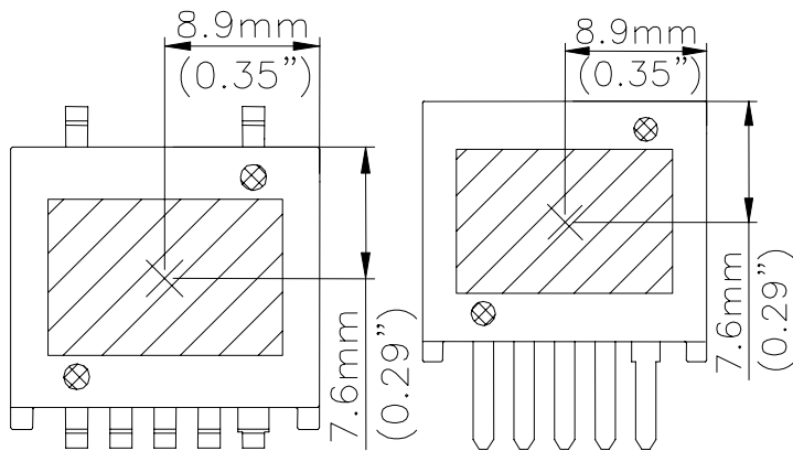
Figure 33: Temperature measurement location
