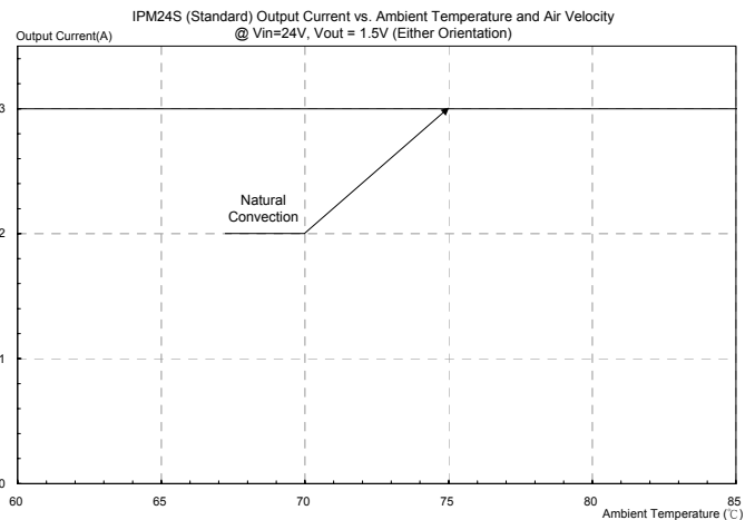
Figure 36: Output current vs. ambient temperature and air velocity @Vin=24V, Vout=1.5V(Either Orientation)
