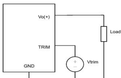
Figure 31: Circuit configuration for programming output voltage using external voltage source
