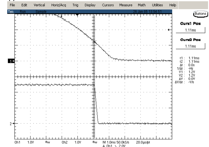
Figure 16: Power off waveform 24vin, 2.5V/3A out with application of Vin
