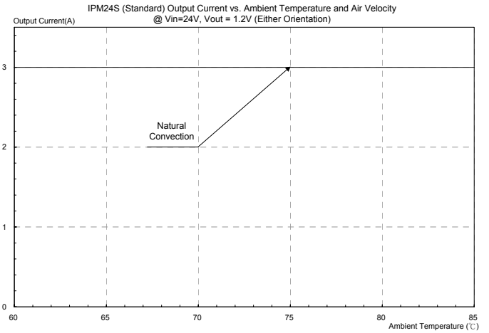
Figure 37: Output current vs. ambient temperature and air velocity @Vin=24V, Vout=1.2V(Either Orientation)
