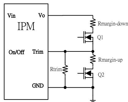
Figure 32: Circuit configuration for output voltage margining
