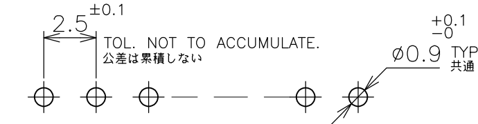
RECOMMENDED BOARD LAYOUT (1.6 THK) 取付基板寸寸法(基板厚 1.6t)
