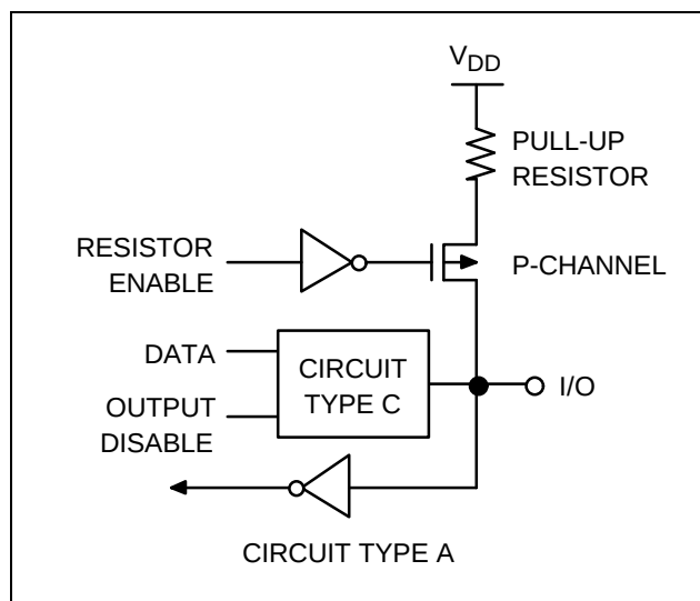
Figure 1-6. Pin Circuit Type D (P0.1, P0.2, P2, P3, P6, P7)
