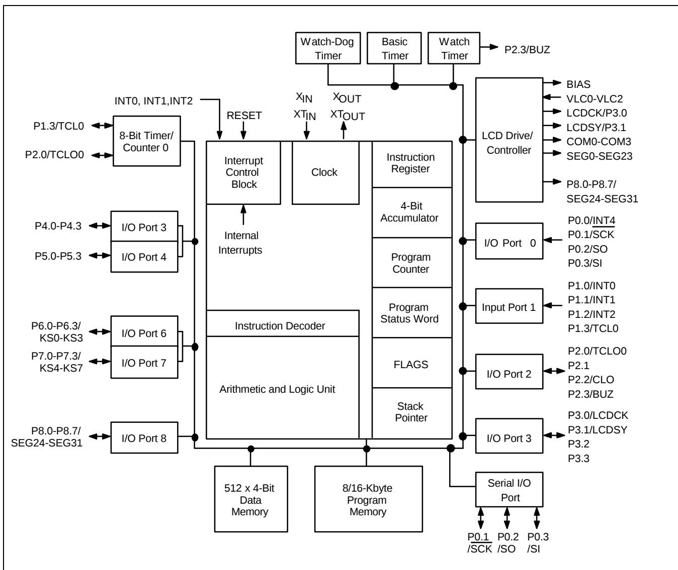
Figure 1-1. S3C7238/C7235 Simplified Block Diagram
