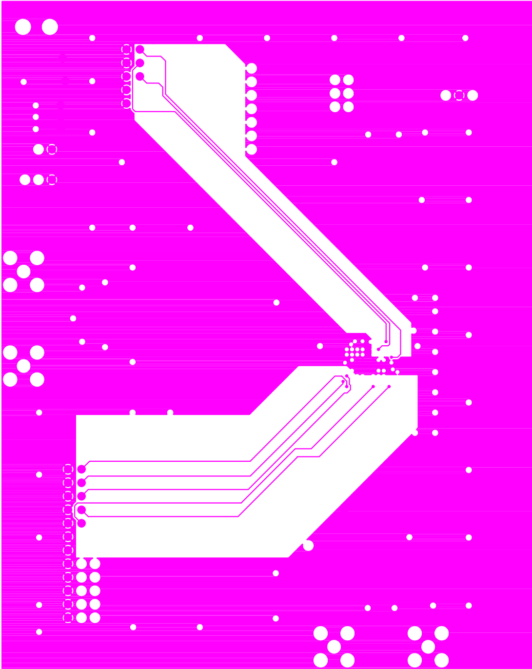
Figure 8. Si5320-EVB—Layer 6, VDD 3.3
