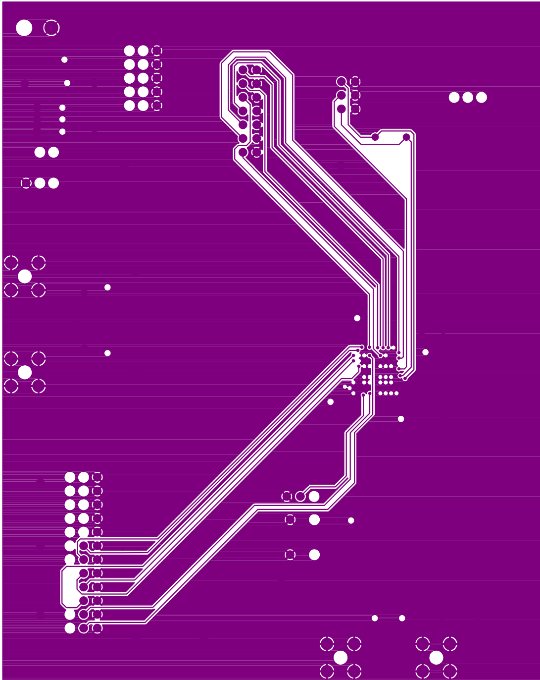
Figure 9. Si5320-EVB—Layer 7, GND
