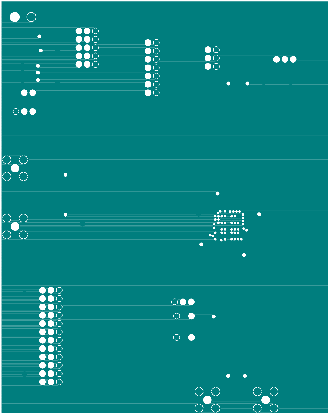
Figure 7. Si5320-EVB—Layer 5, GND
