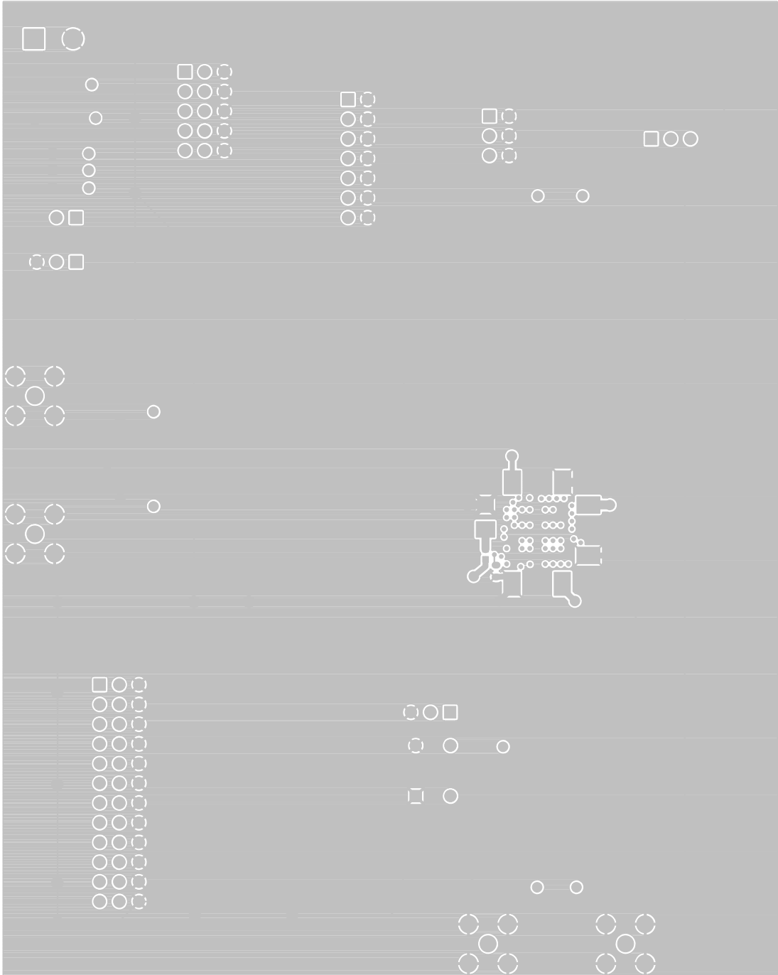
Figure 10. Si5320-EVB—Layer 8, Bottom
