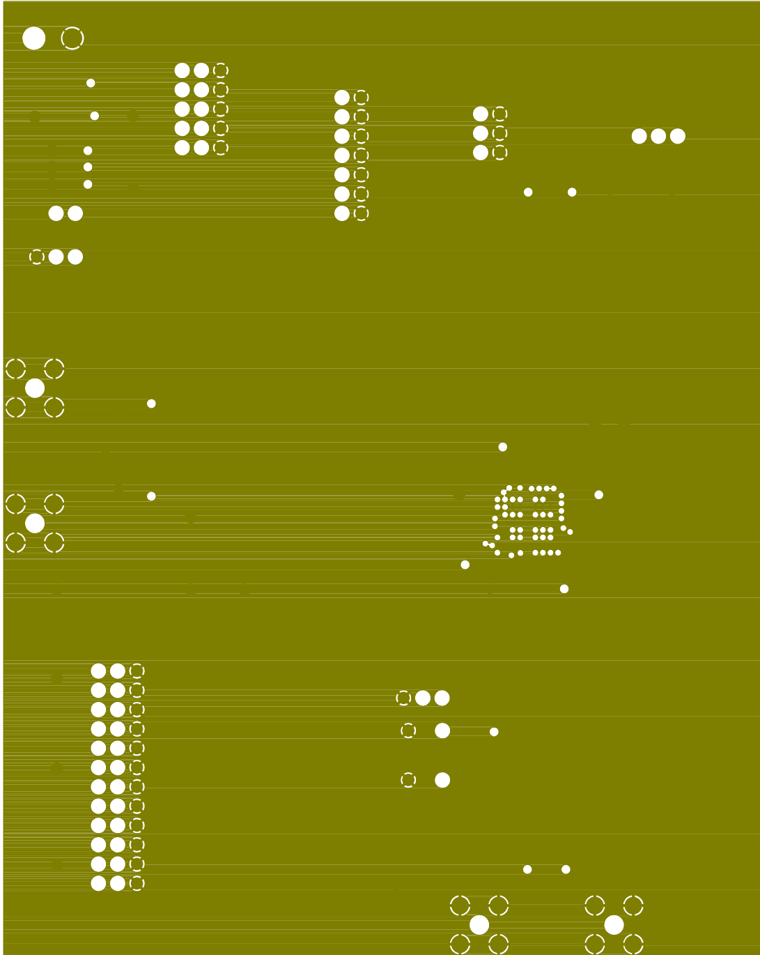
Figure 5. Si5320-EVB—Layer 3, GND
