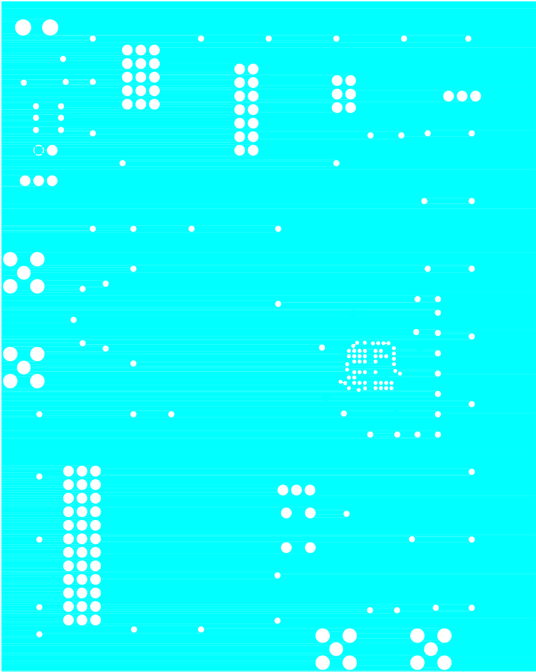
Figure 6. Si5320-EVB—Layer 4, VDD 2.5
