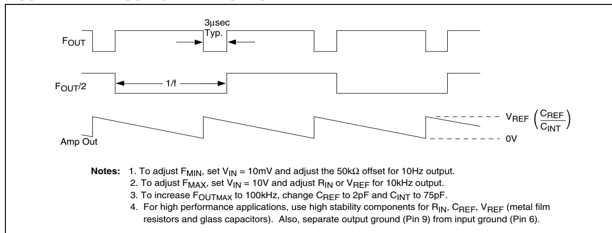
FIGURE 4-1: OUTPUT WAVEFORMS
