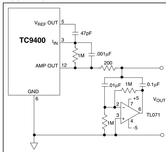
FIGURE 7-5: RIPPLE FILTER
