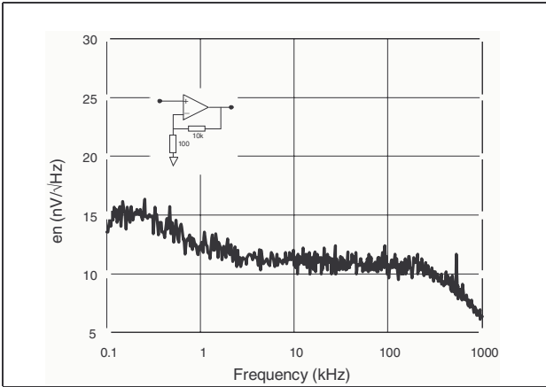
Figure 26. Equivalent noise voltage
