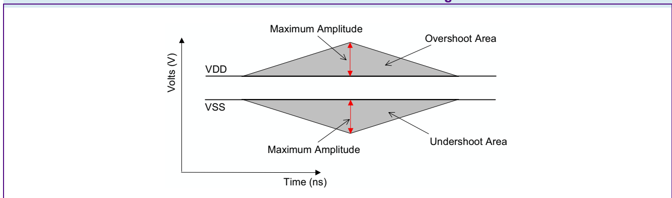
AC Overshoot / Undershoot Diagram for Address and Control Pins
