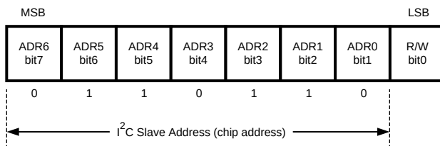
Figure 7. Chip Address
