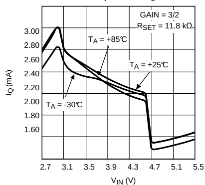
Quiescent Current in Gain 1.5×
