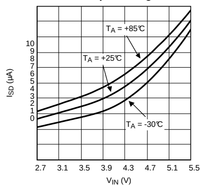
Shutdown Current
