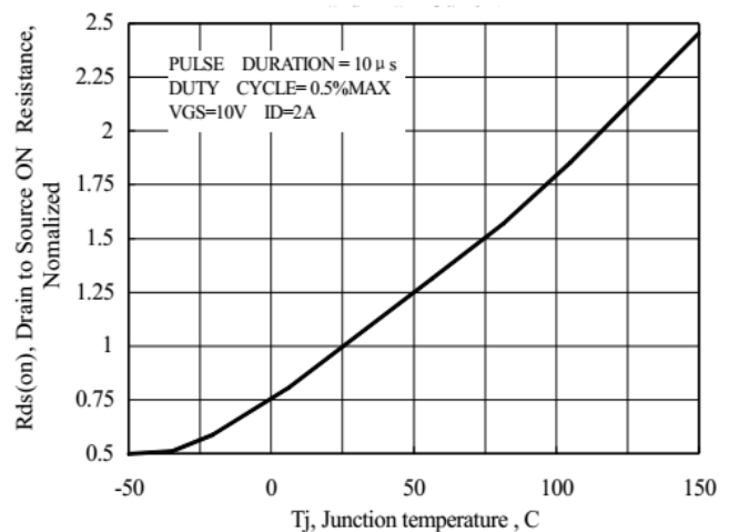
Figure 10 Typical Drilan to Source on Resistance vs Junction Temperature
