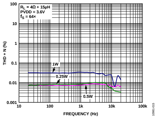
Figure 12. THD + N vs. Frequency, PVDD = 3.6 V, R_L = 4\ \Omega , f_S = 64\times
