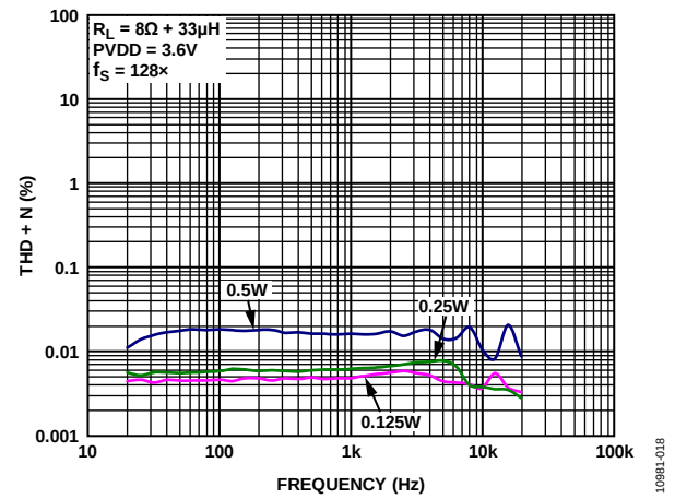
Figure 15. THD + N vs. Frequency, PVDD = 3.6 V, R_L = 8\ \Omega , f_S = 128\times
