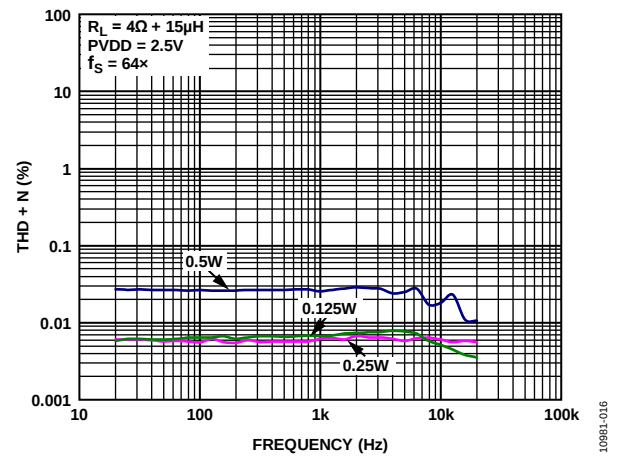
Figure 13. THD + N vs. Frequency, PVDD = 2.5 V, R_L = 4\ \Omega , f_S = 64\times
