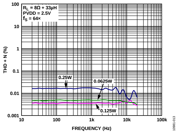
Figure 10. THD + N vs. Frequency, PVDD = 2.5 V, R_L = 8\ \Omega , f_S = 64\times
