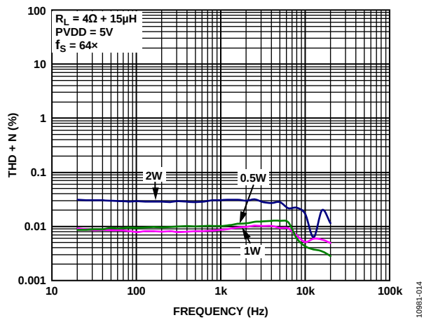
Figure 11. THD + N vs. Frequency, PVDD = 5 V, R_L = 4\ \Omega , f_S = 64\times
