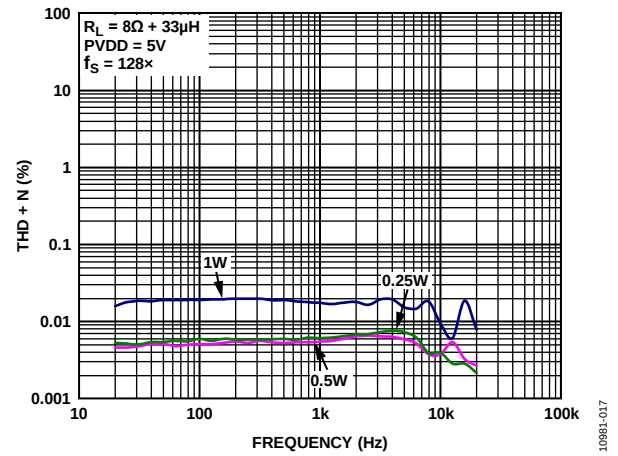
Figure 14. THD + N vs. Frequency, PVDD = 5 V, R_L = 8\ \Omega , f_S = 128\times
