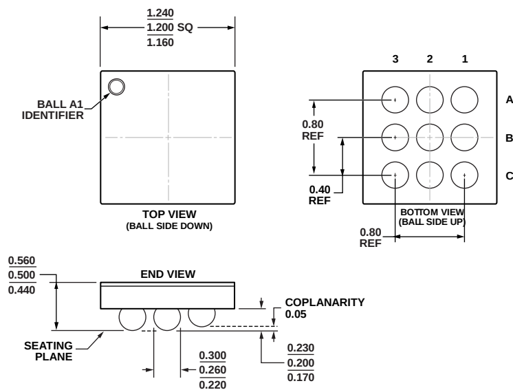
Figure 34. 9-Ball Wafer Level Chip Scale Package [WLCSP] (CB-9-5)
