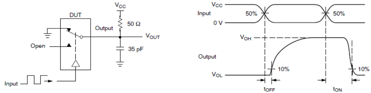
Figure 8. t_{ON} / t_{OFF}
