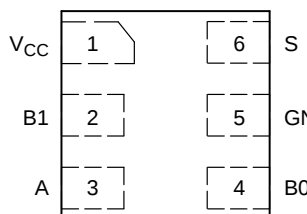
Figure 1. ULLGA6 (NLAS3157) (Top View)
