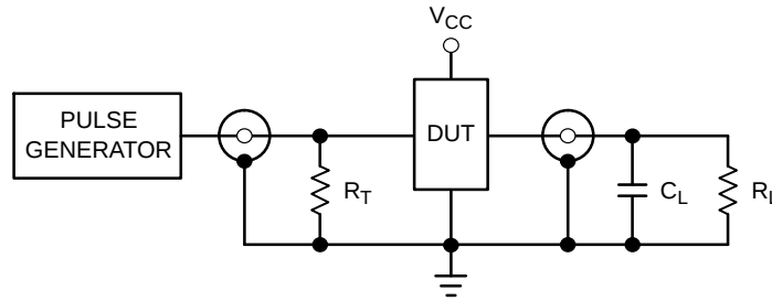
Figure 5. Propagation Delay Test Circuit
