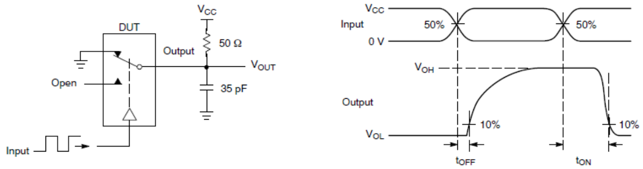
Figure 7. t_{ON} / t_{OFF}
