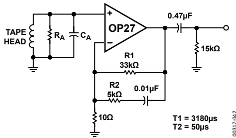
Figure 42. Tape Head Preamplifier
