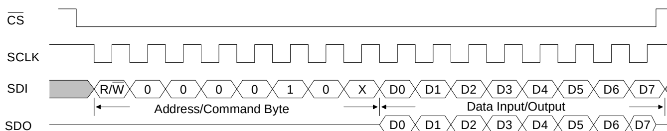
Figure 13. Input/Output Timing
