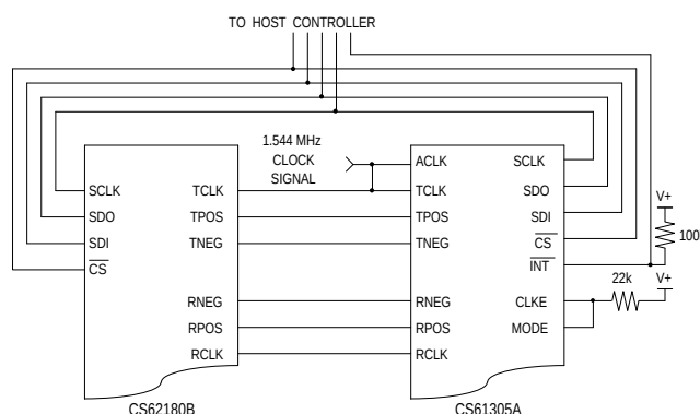
Figure A5. Interfacing the CS61305A with a CS62180B (Host Mode)
