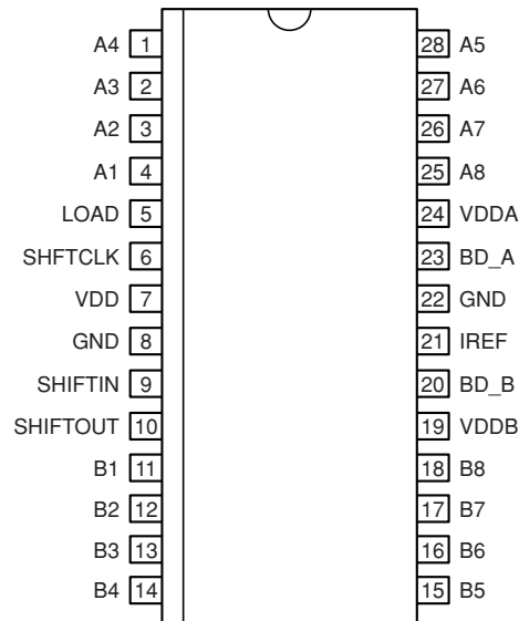
28-Lead SOIC
