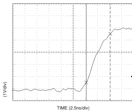
Output Current Sink Fall Time
