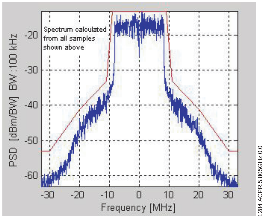
FIGURE 11: SPECTRUM MASK @ POUT = 21 dBm WITH FREQUENCY = 5.805 GHz AND ICC = 215 mA
