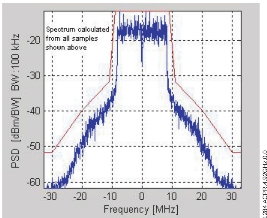
FIGURE 8: SPECTRUM MASK @ POUT = 21 dBm WITH FREQUENCY = 4.92 GHz AND ICC = 235 mA
