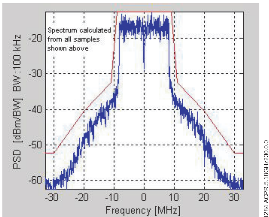
FIGURE 9: SPECTRUM MASK @ POUT = 21 dBm WITH FREQUENCY = 5.18 GHz AND ICC = 230 mA
