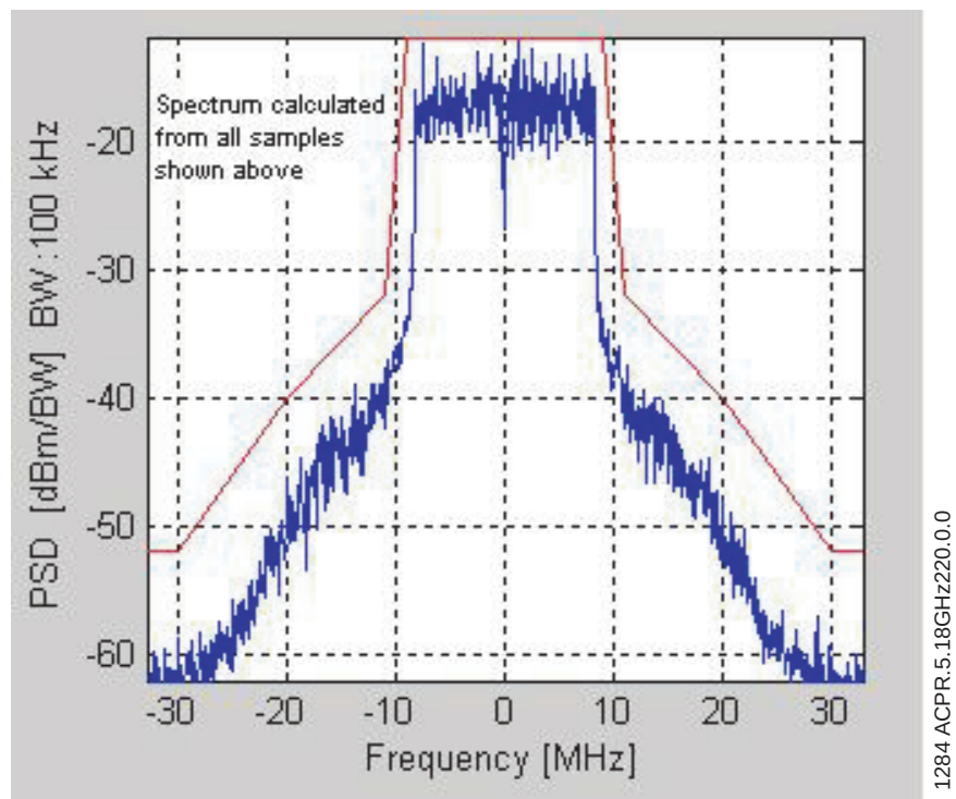
FIGURE 10: SPECTRUM MASK @ POUT = 21 dBm WITH FREQUENCY = 5.32 GHz AND ICC = 220 mA
