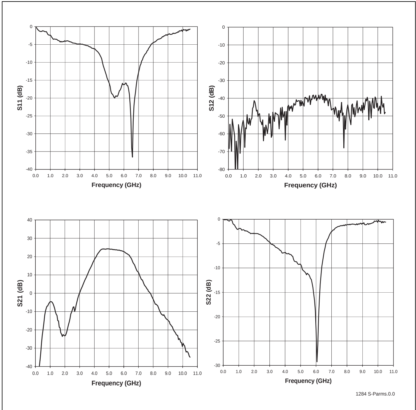
FIGURE 2: S-PARAMETERS
