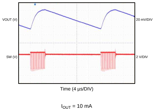
Figure 7. Output Voltage Ripple in ECO Mode
