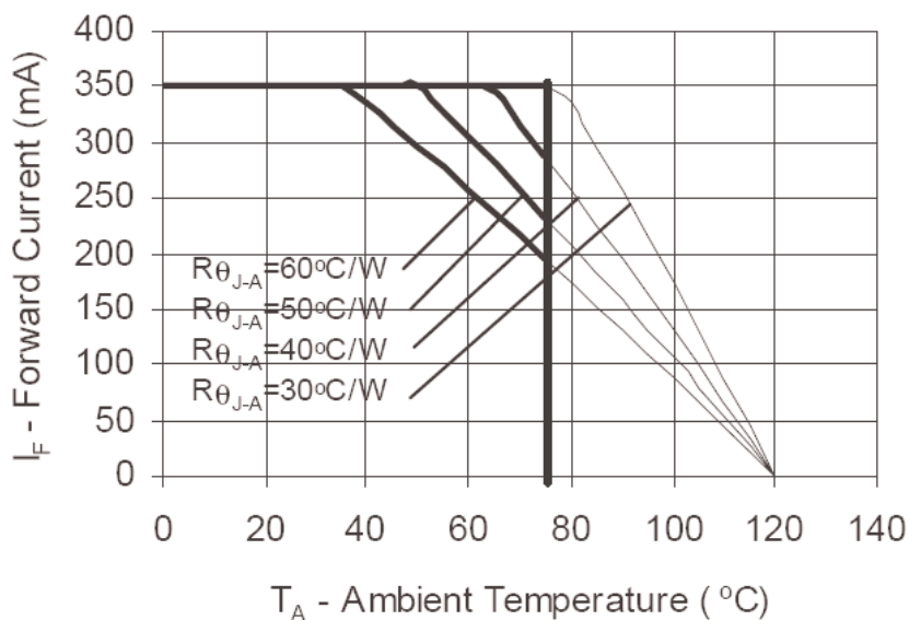
Figure 4b. Maximum Forward Current vs. Ambient Temperature. Derating based on T_{JMAX} = 120^{\circ}\text{C} and T_{\text{AMBIENT MAX}} = 75^{\circ}\text{C} for LXHLNWG8.
