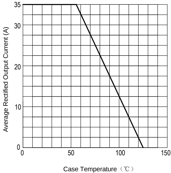
FIG1:Io-Tc Curve
