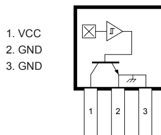
Package UA, 3-pin SIP
