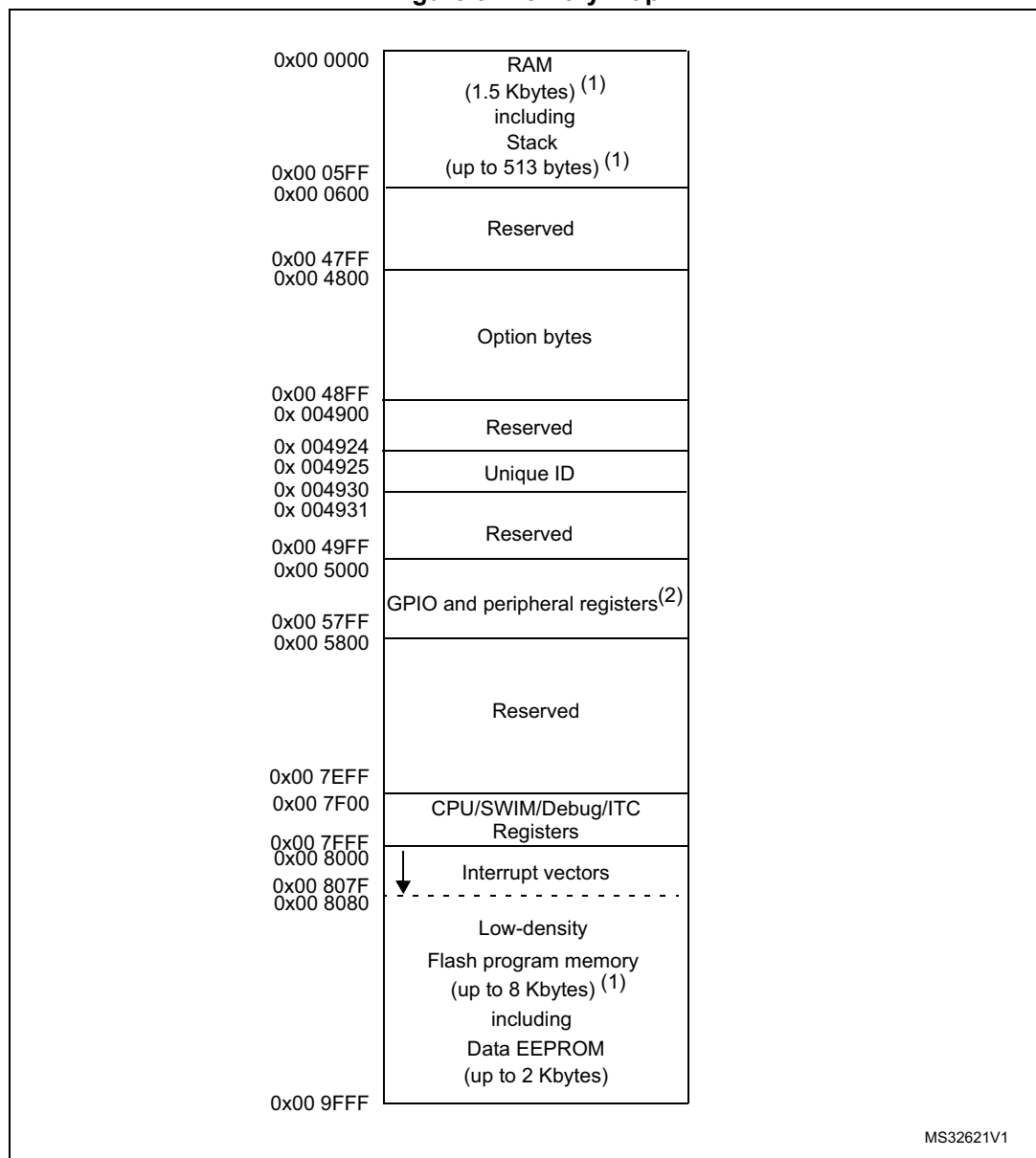
Figure 3. Memory map
