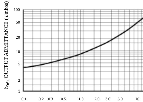
Figure 12. Output Admittance
