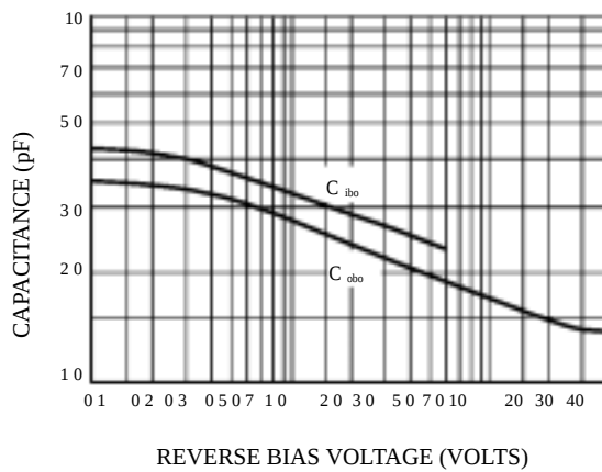
Figure 3. Capacitance
