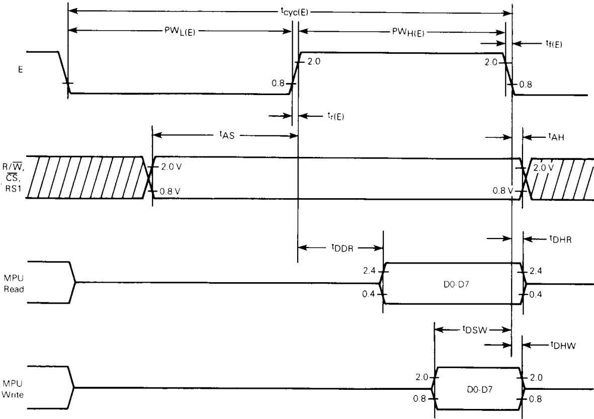
FIGURE 1 — BUS TIMING
