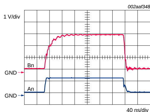
Fig 14. Example of typical AC waveform
