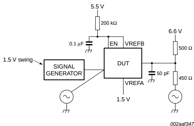
Fig 13. AC test setup
