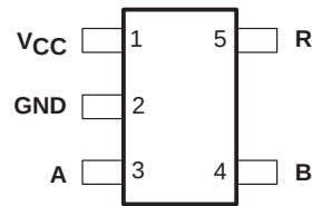
SN65LVDT2 DBV PACKAGE (TOP VIEW)
