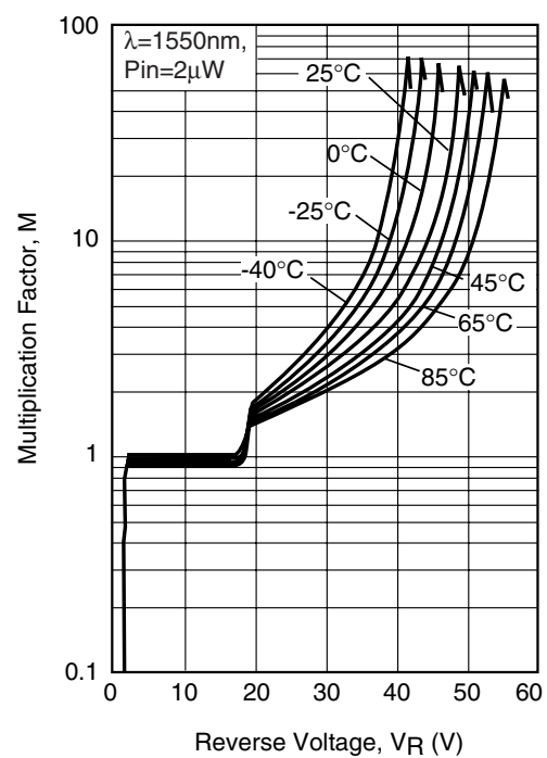
Fig. 5 Multiplication Characteristics
