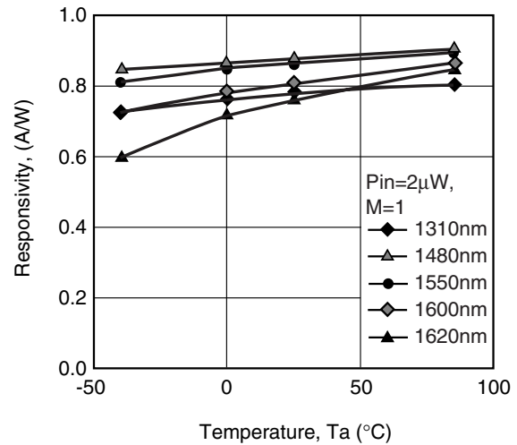
Fig. 2 Responsivity vs. Temperature
