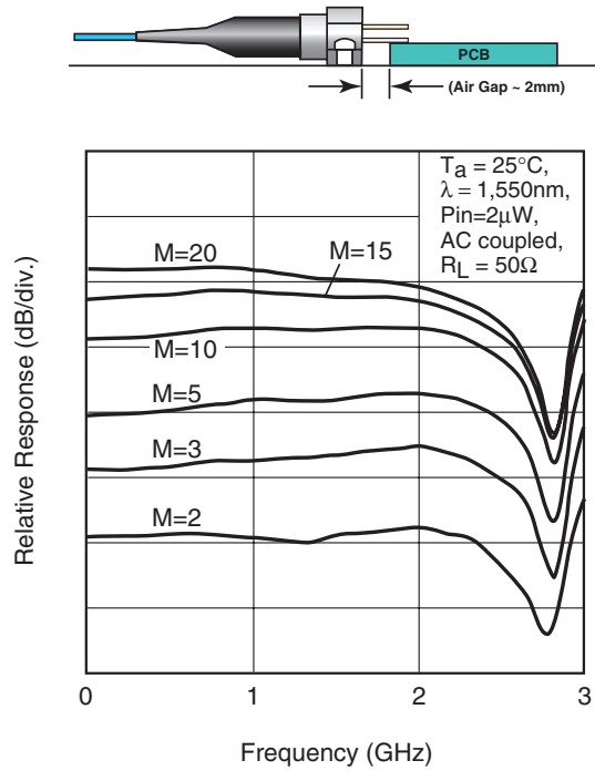
Fig. 7A Frequency Response (Air Gap ~ 2mm)
