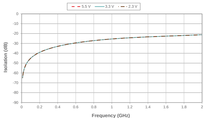
Figure 11 • Isolation vs V_{DD} (RFC–RFX)
