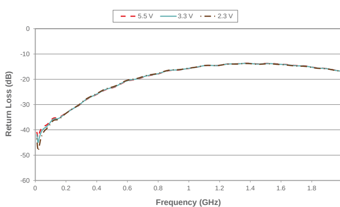
Figure 7 • RFX Port Return Loss vs V_{DD}
