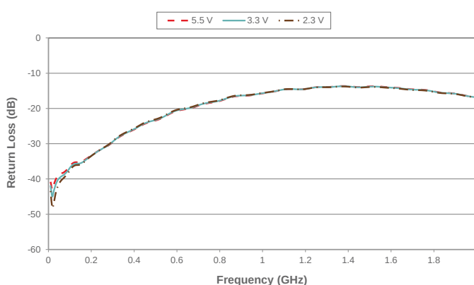
Figure 7 • RFX Port Return Loss vs V_{DD}
