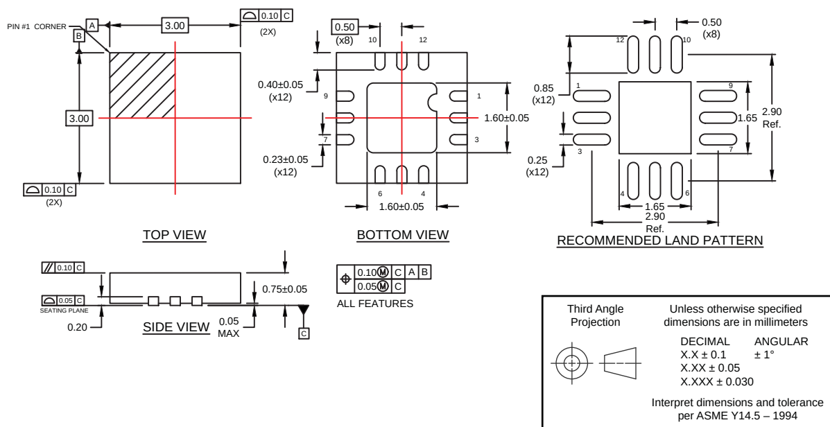
Figure 14 • Package Mechanical Drawing for 12-lead 3 \times 3 \times 0.75 mm QFN
