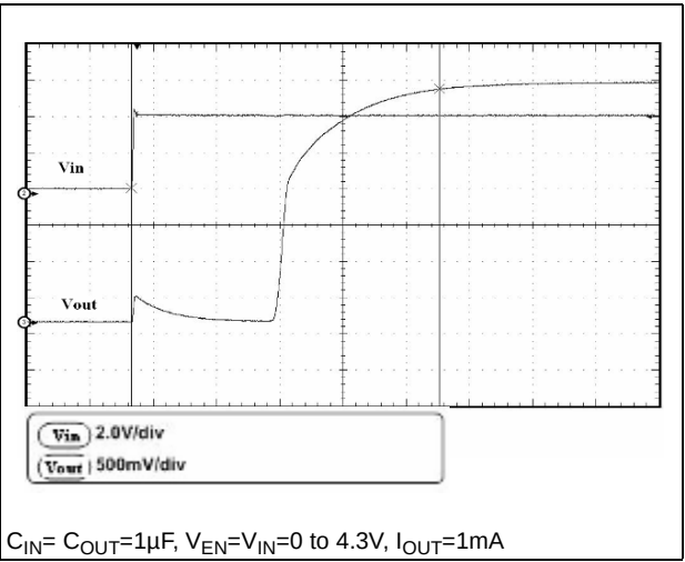
Figure 13. Enable transient
