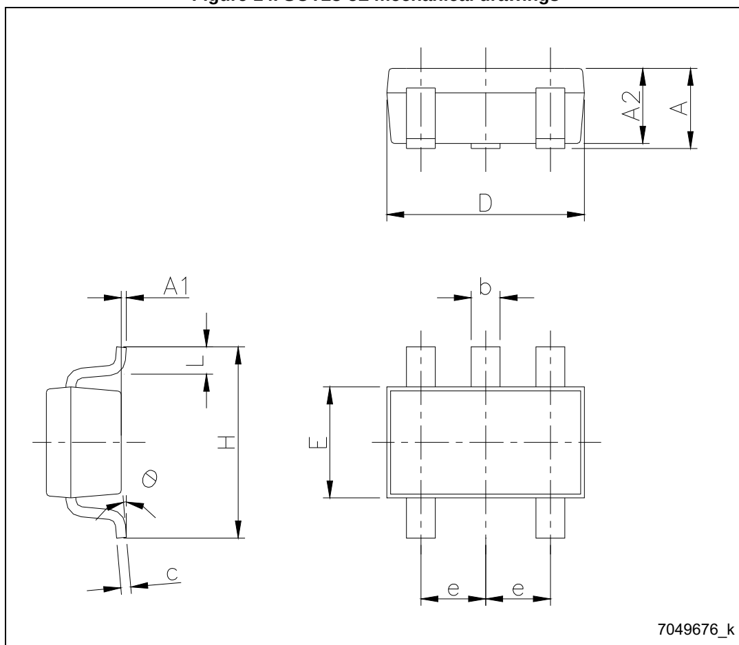
Figure 14. SOT23-5L mechanical drawings
