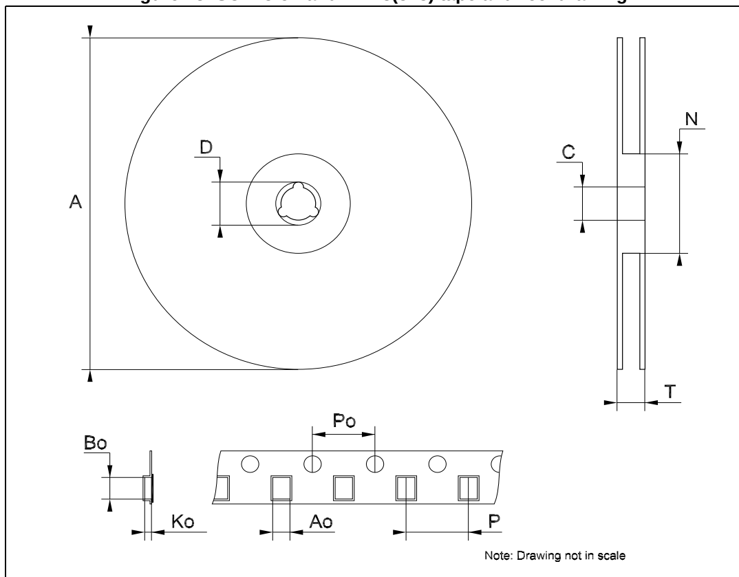
Figure 18. SOT23-5L and DFN8(3x3) tape and reel drawing
