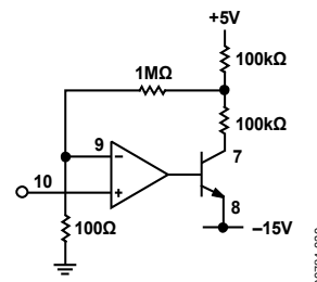
Figure 26. Comparator Hysteresis
