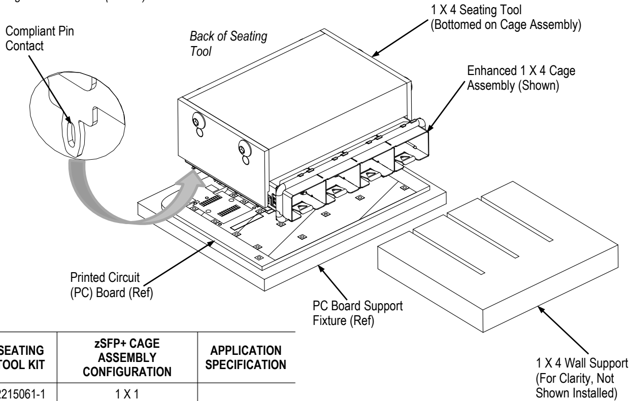
Seating Tool 2215061-1 (Shown)
