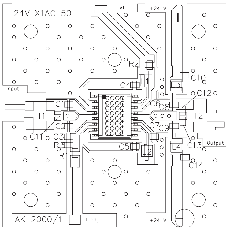
Figure 13: Evaluation Board Layout
