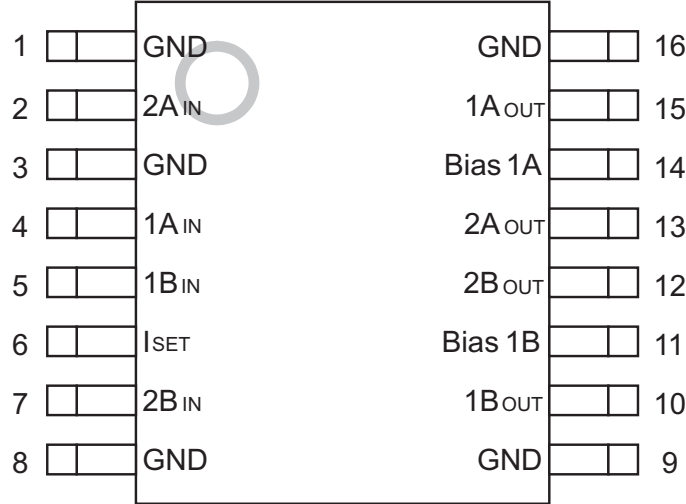
Figure 2: Pin Out
