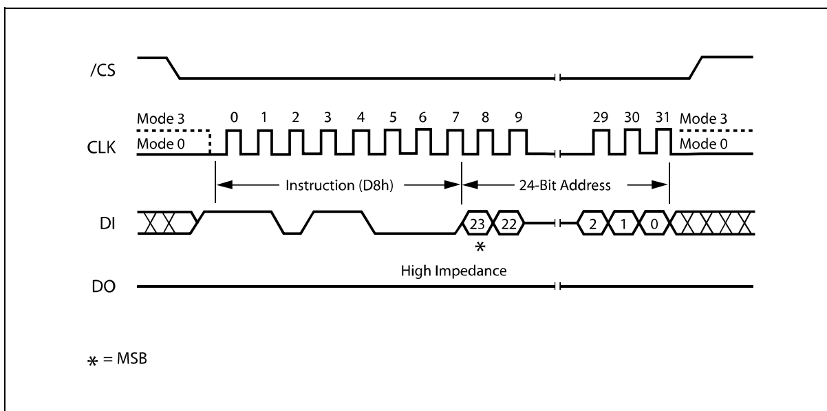
Figure 23. 64KB Block Erase Instruction Sequence Diagram
