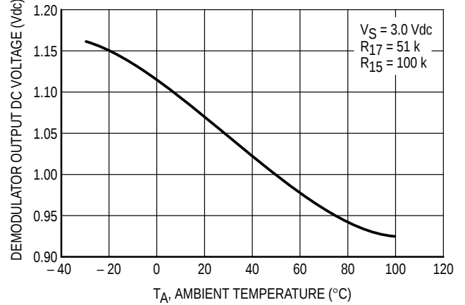
Figure 11. Demodulator DC Voltage versus Ambient Temperature
