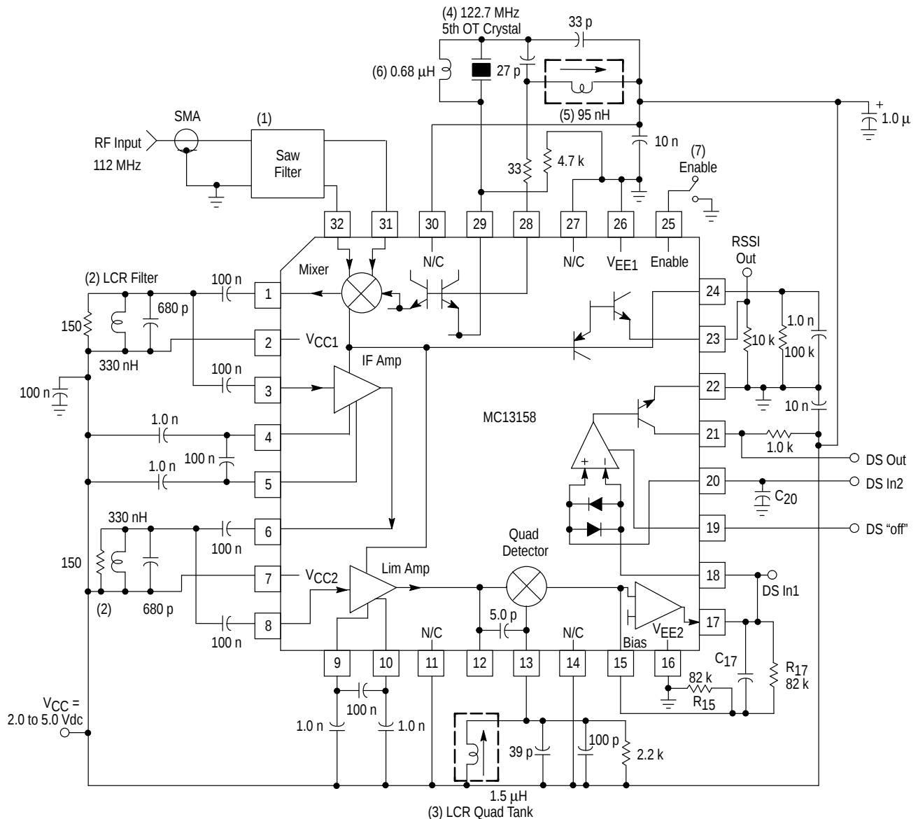
Figure 12. Application Circuit
