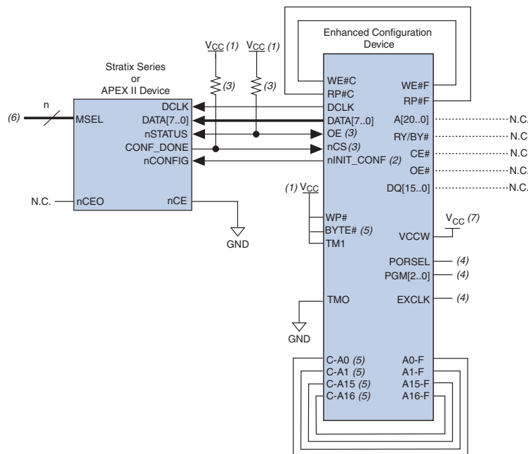
Figure 1-2. FPP Configuration
