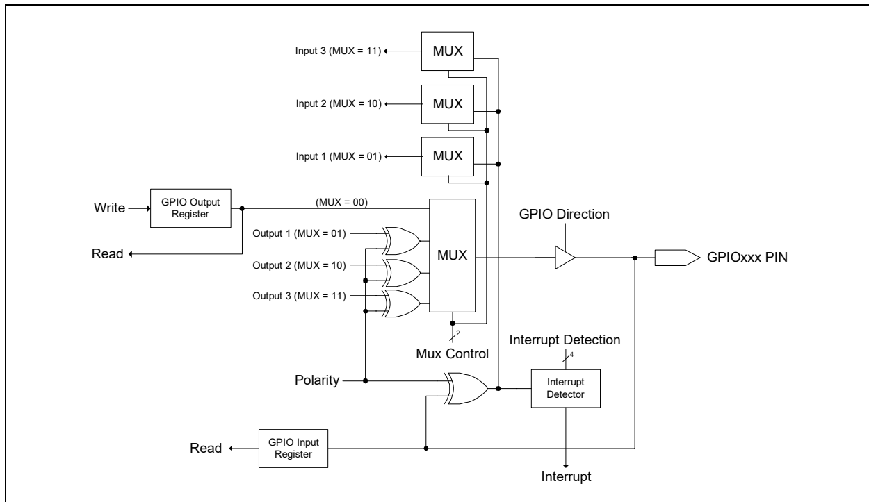
FIGURE 11-1: GPIO INTERFACE BLOCK DIAGRAM
