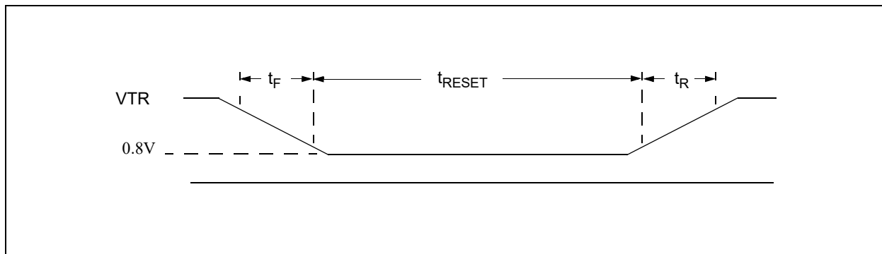
FIGURE 34-3: NRESET_IN TIMING
