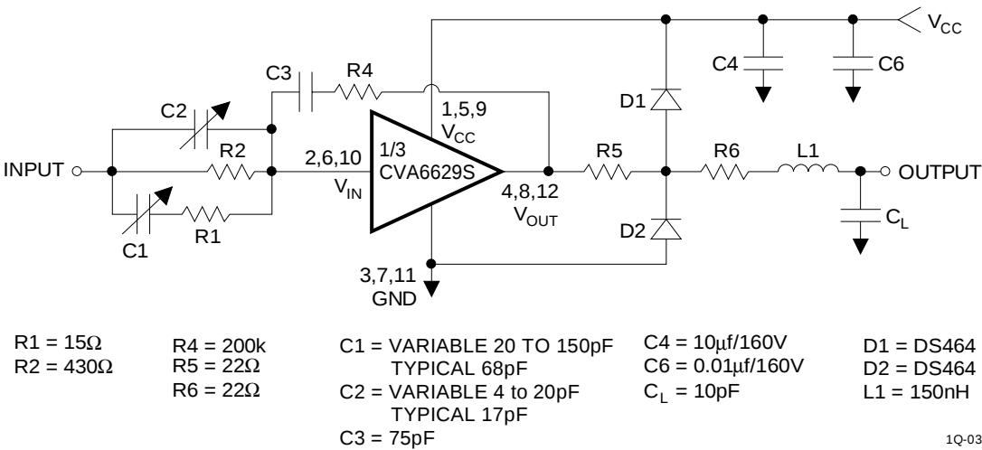
FIGURE 1. TEST CIRCUIT
