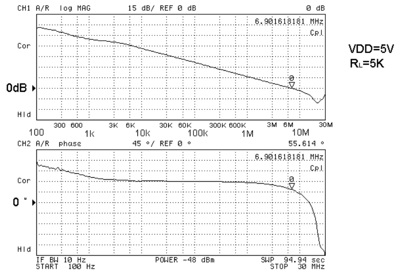
Open Loop Frequency Response
