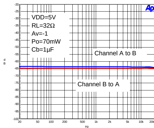
Channel Separation
