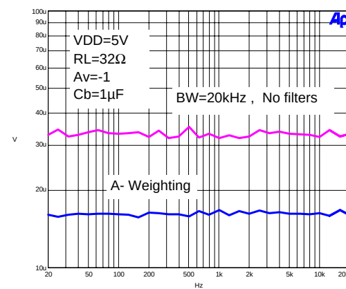
Output Noise
