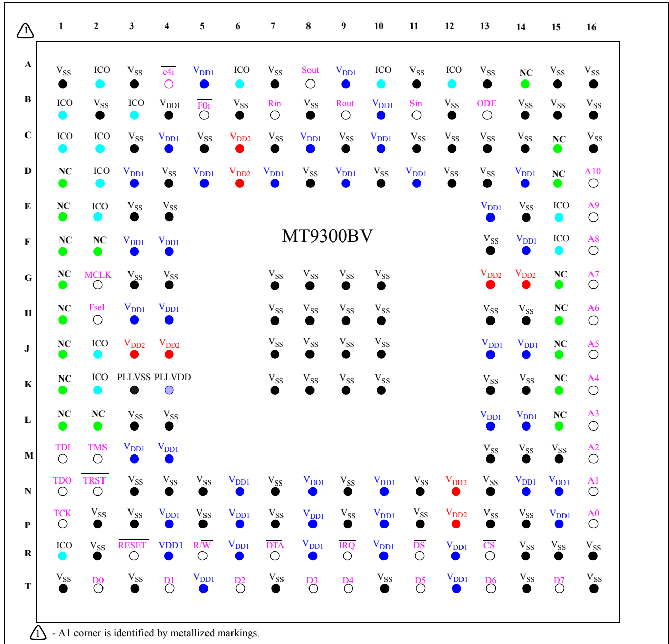
Figure 2 - 208 Ball LGA
