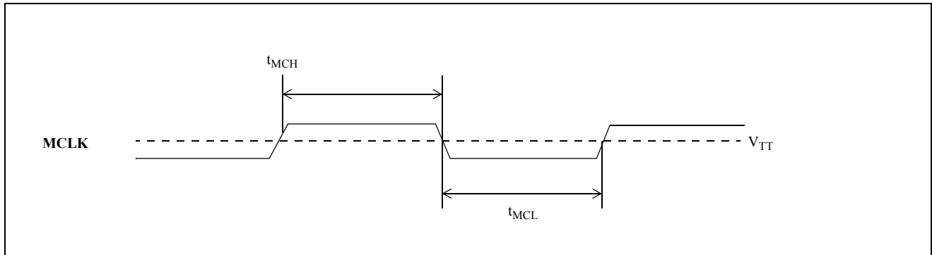
Figure 13 - Master Clock
