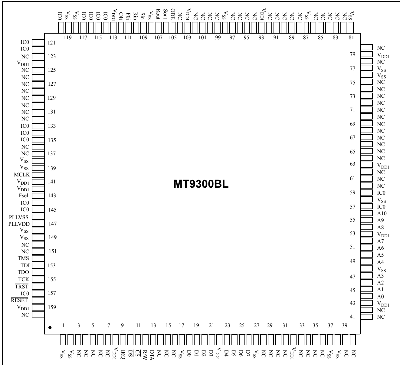
Figure 3 - 160 Pin MQFP
