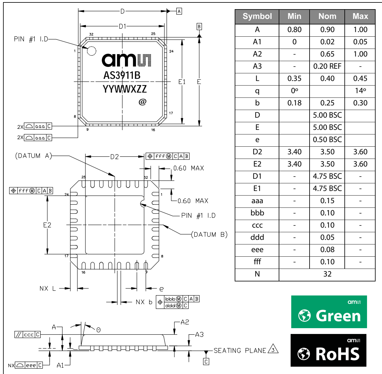
Figure 130: Package Drawings
