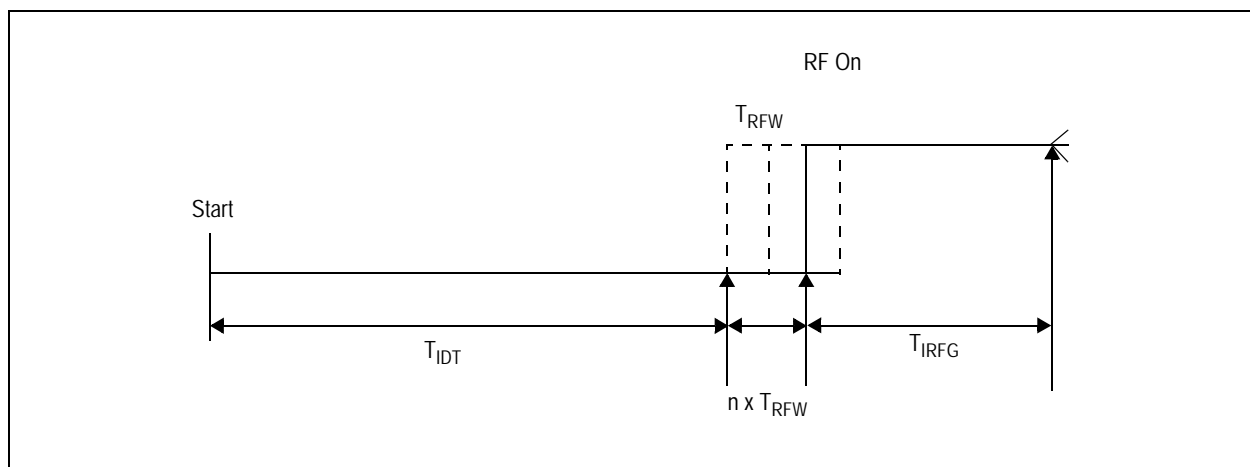
Figure 36: Direct Command NFC Initial Field ON
