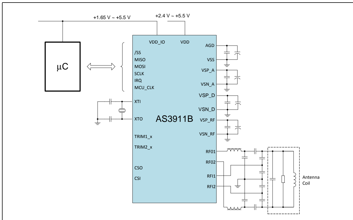
Figure 11: Minimum Configuration with Differential Antenna Driving Including EMC Filter
