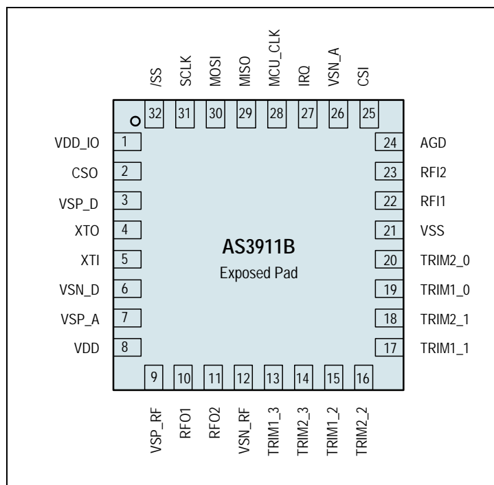
Figure 3: Pin Diagram
