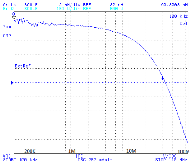
PI13067-R10
