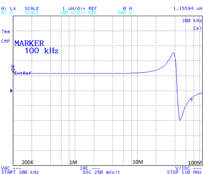
PI13067-1R2
