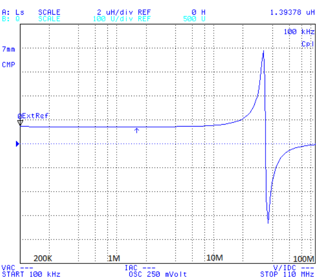
PI13067-1R5
