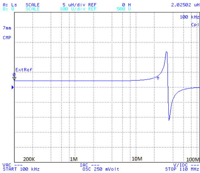
PI13067-4R7
