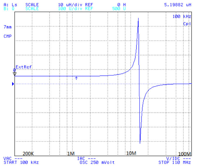
PI13067-8R2
