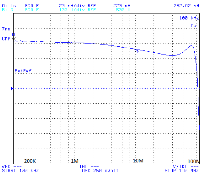
PI13067-R30
