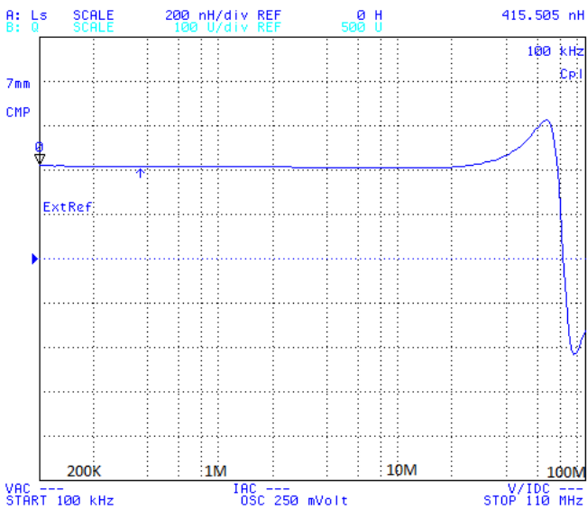
PI13067-R40
