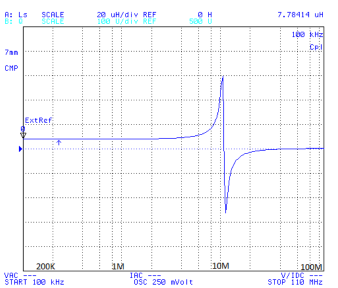
PI13067-8R2
