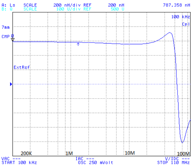
PI13067-R82
