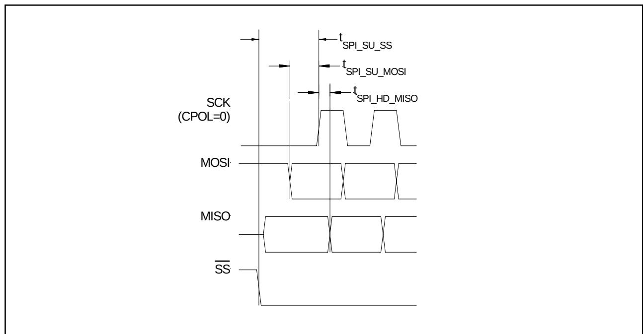
Fig. 3: Timing characteristics
