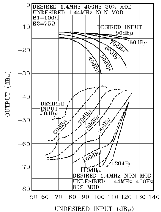
CROSS MODULATION CHARACTERISTIC
